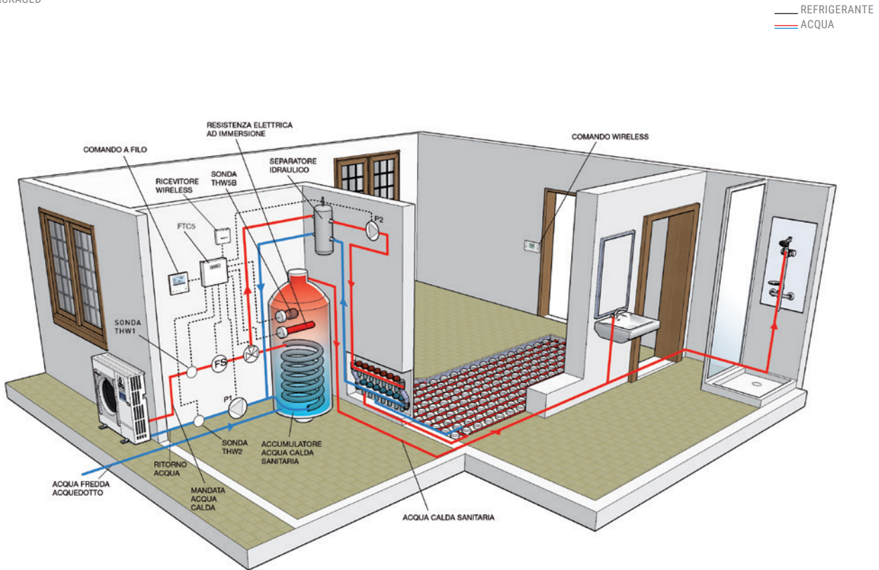
SCHEMA PACKAGED
